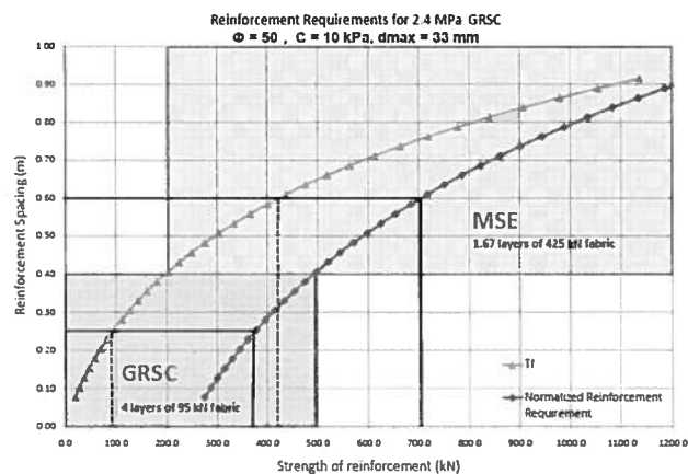
Fig. 4 Example of reinforcement requirements based on GRSC behaviour
